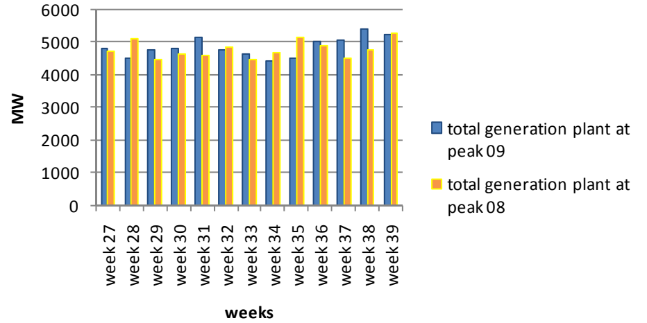
Total Generation at Peak Q3 2009 vs Q3 2008
