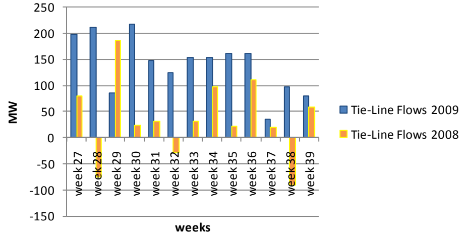
Tie-Line Flows SONI to EirGrid Q3 2009 vs 2008
