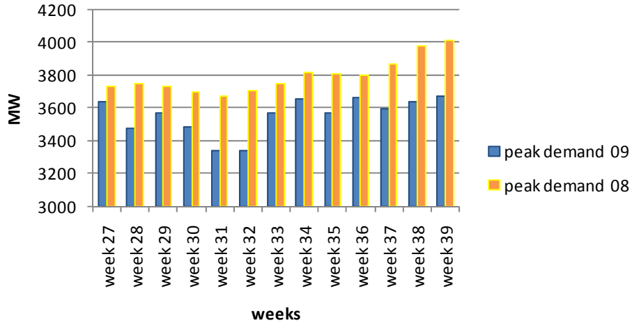
Peak Demand Q3 2009 vs Q3 2008
